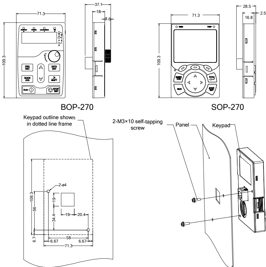
Dimension and hole sizes for mounting keypad without a bracket
